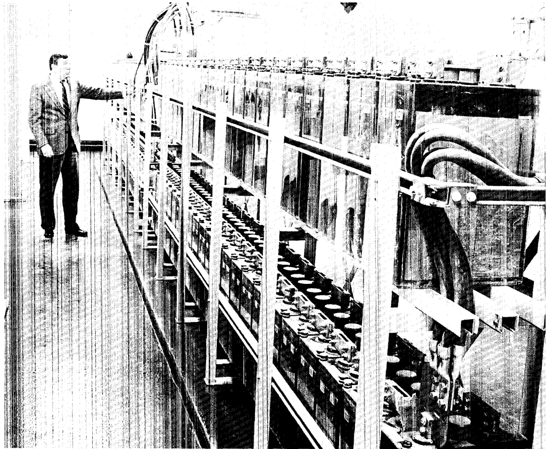
The Annapolis Data Center not only races against Father Time in its operations but it will be able to handle Mother Nature with an uninterruptible power supply. In case of commercial power loss, special batteries inspected by Tony Moen immediately relay current — followed by the full support of a diesel generator.
